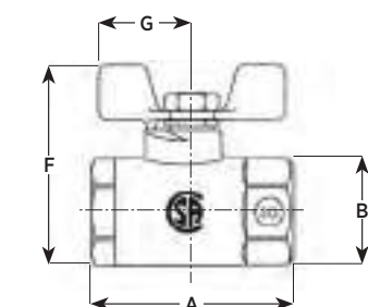
STANDARD - YELLOW DIE-CAST ZINC "WING HANDLE"
