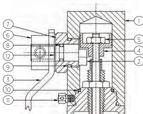
PACKED LEVER
