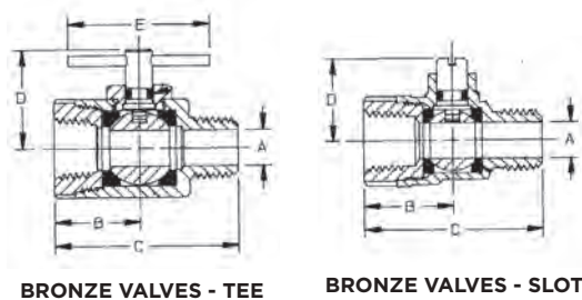
78LF-290: BRONZE
