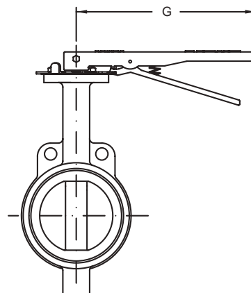
WITH HANDLE
